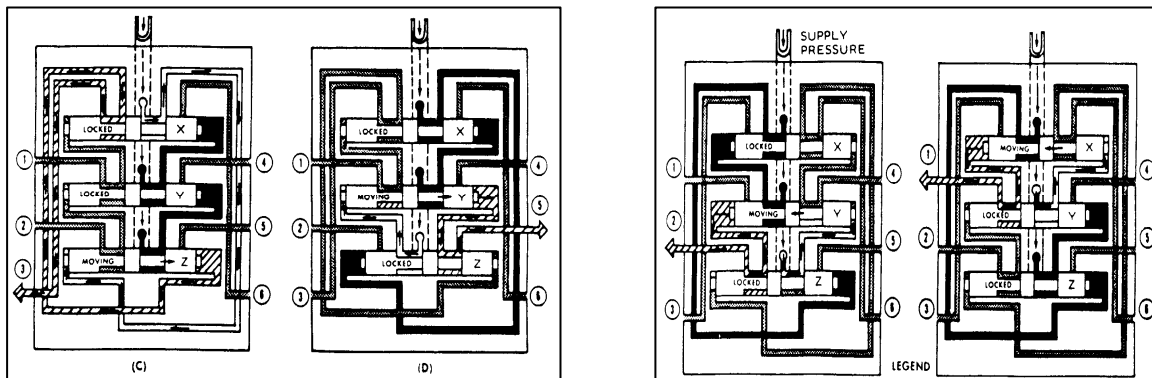
Principle drawing
